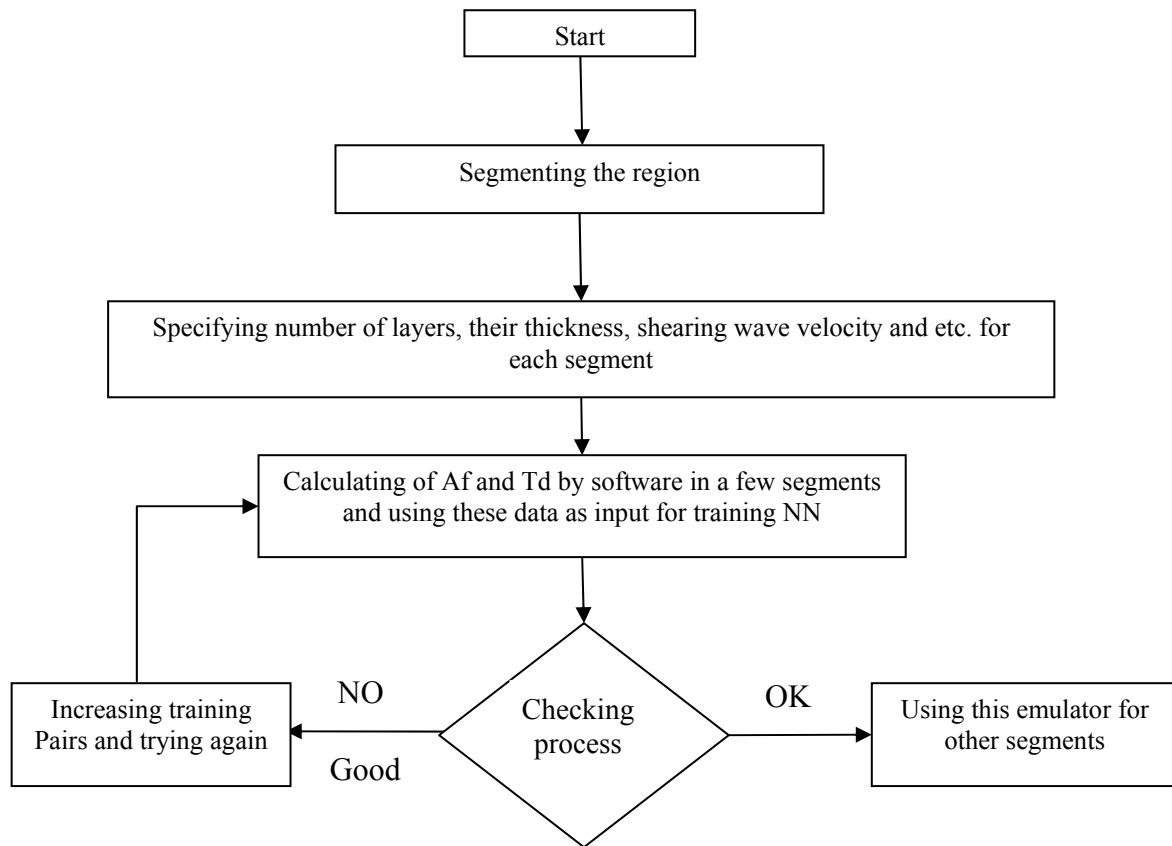
Flowchart 1: Recommended method for determining A_f and T_d by using neural network
