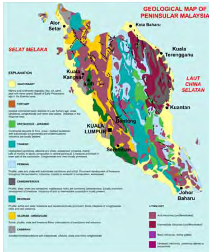
Figure 2: Geological map of Peninsular Malaysia
