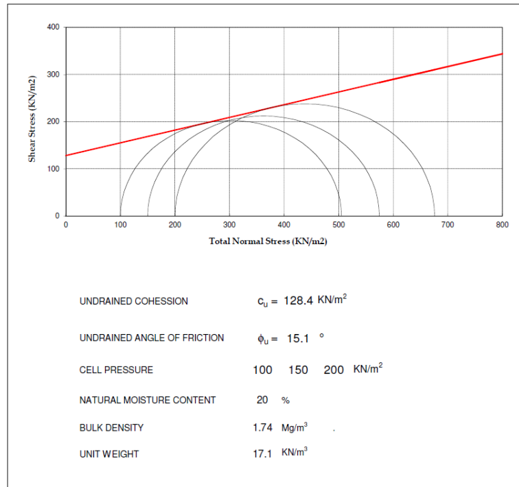
Figure 6: Stress Envelope for Test on BH 3.
