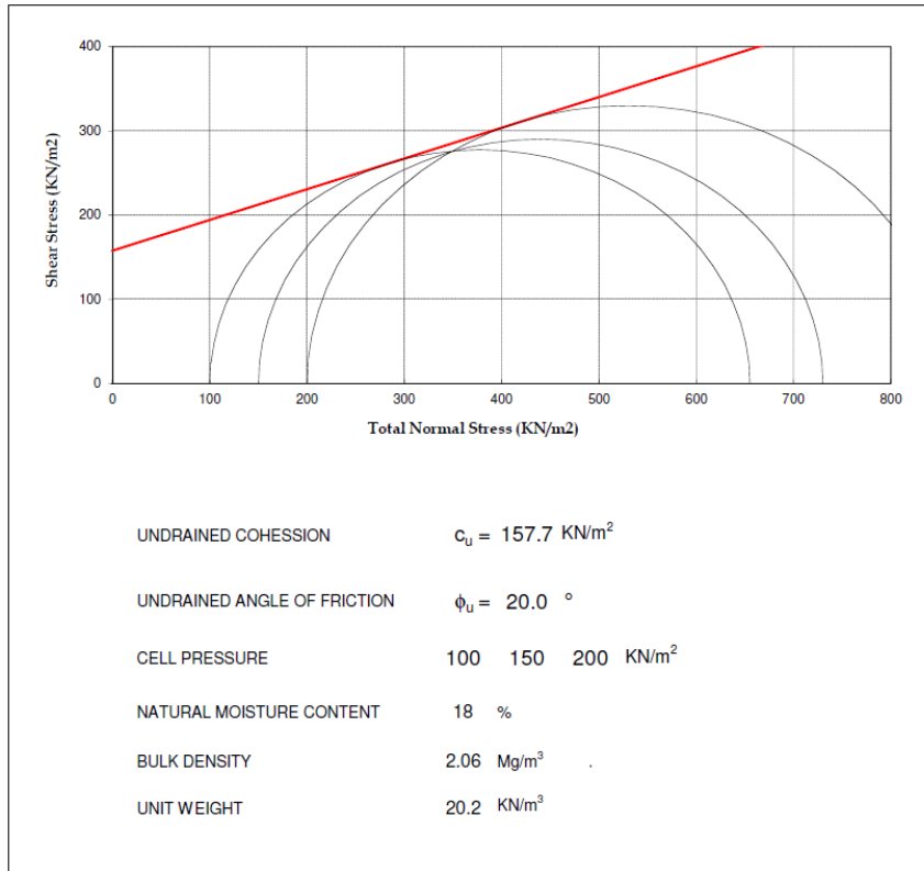
Figure 5: Stress Envelope for Test on BH 2.
