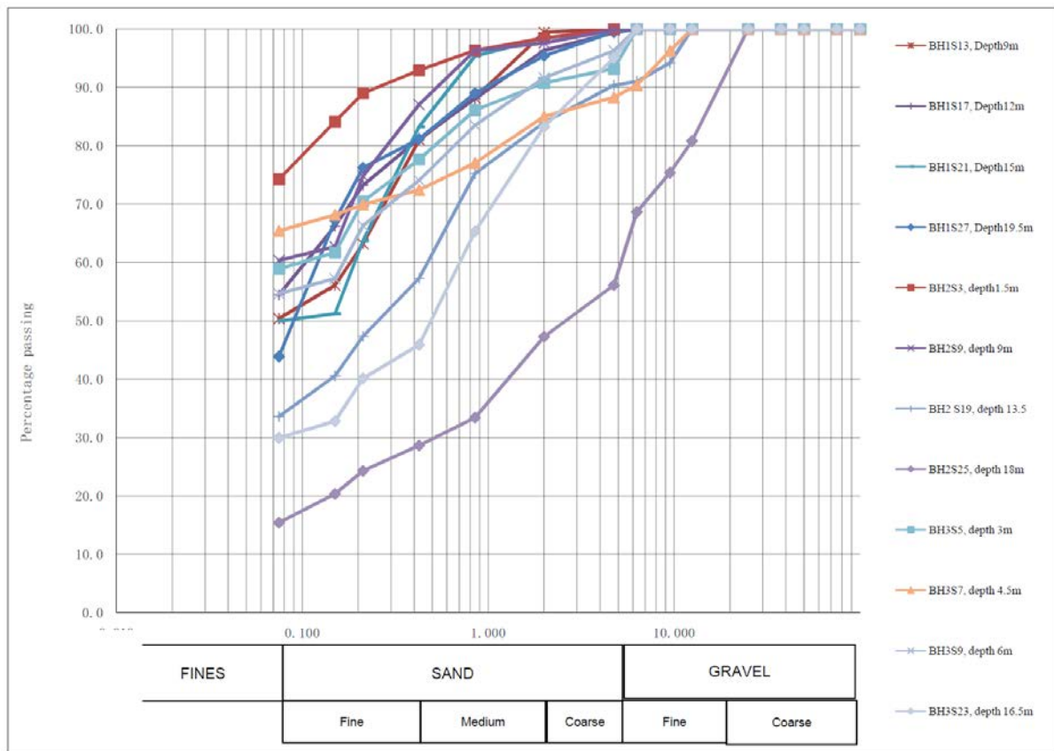
Figure 3: Particle Size Distribution of Samples (selected)
