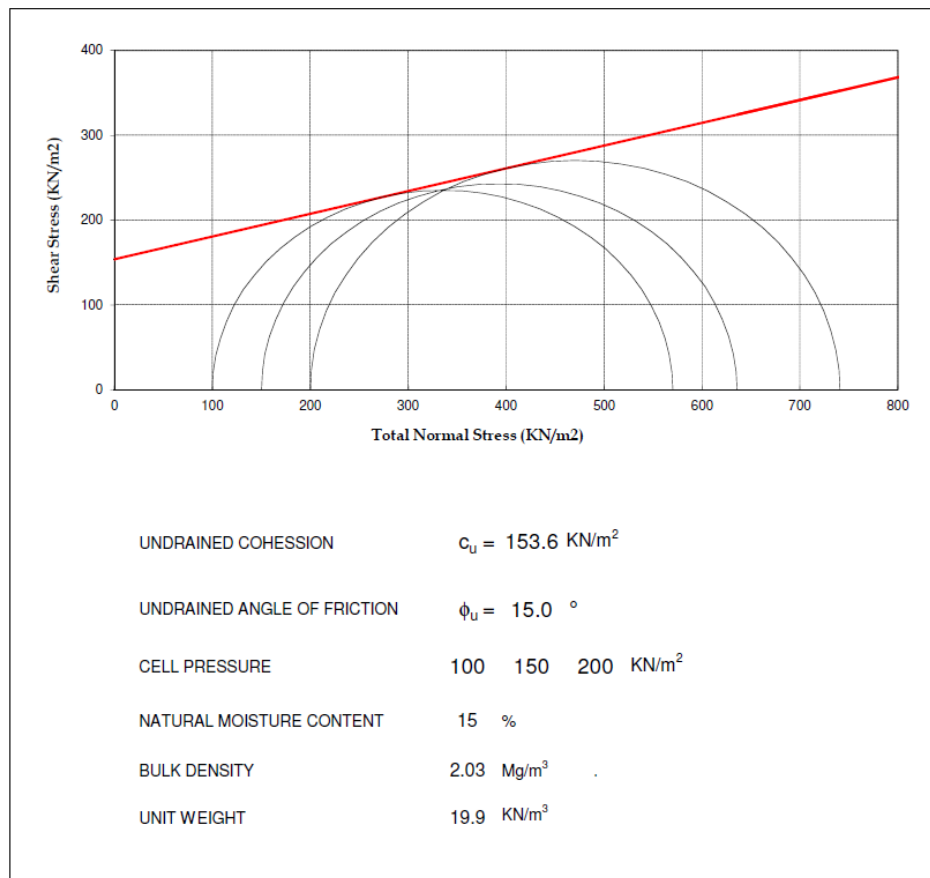
Figure 4: Stress Envelope for Test on BH 1.
