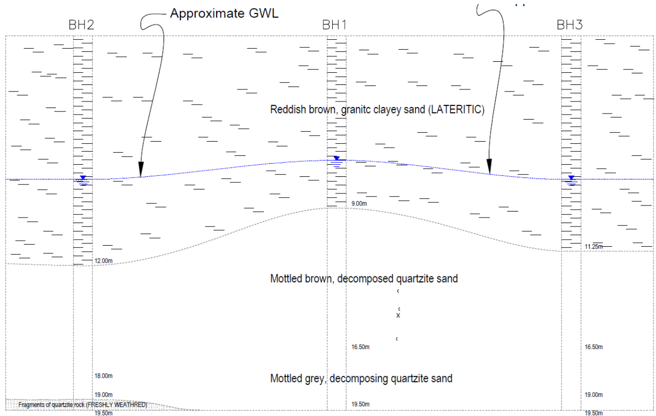
Figure 7: Stratigraphic Description of the Soil Profile.
