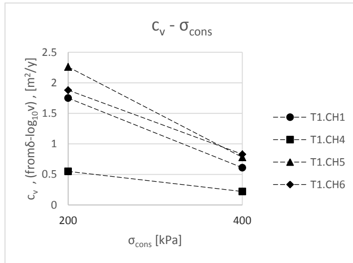
Figure 3: Variation of coefficient of consolidation obtained from d\delta/dt-\delta , \delta-d\delta/dt , \delta-\log_{10}(d\delta/dt) curves with consolidation pressure.
