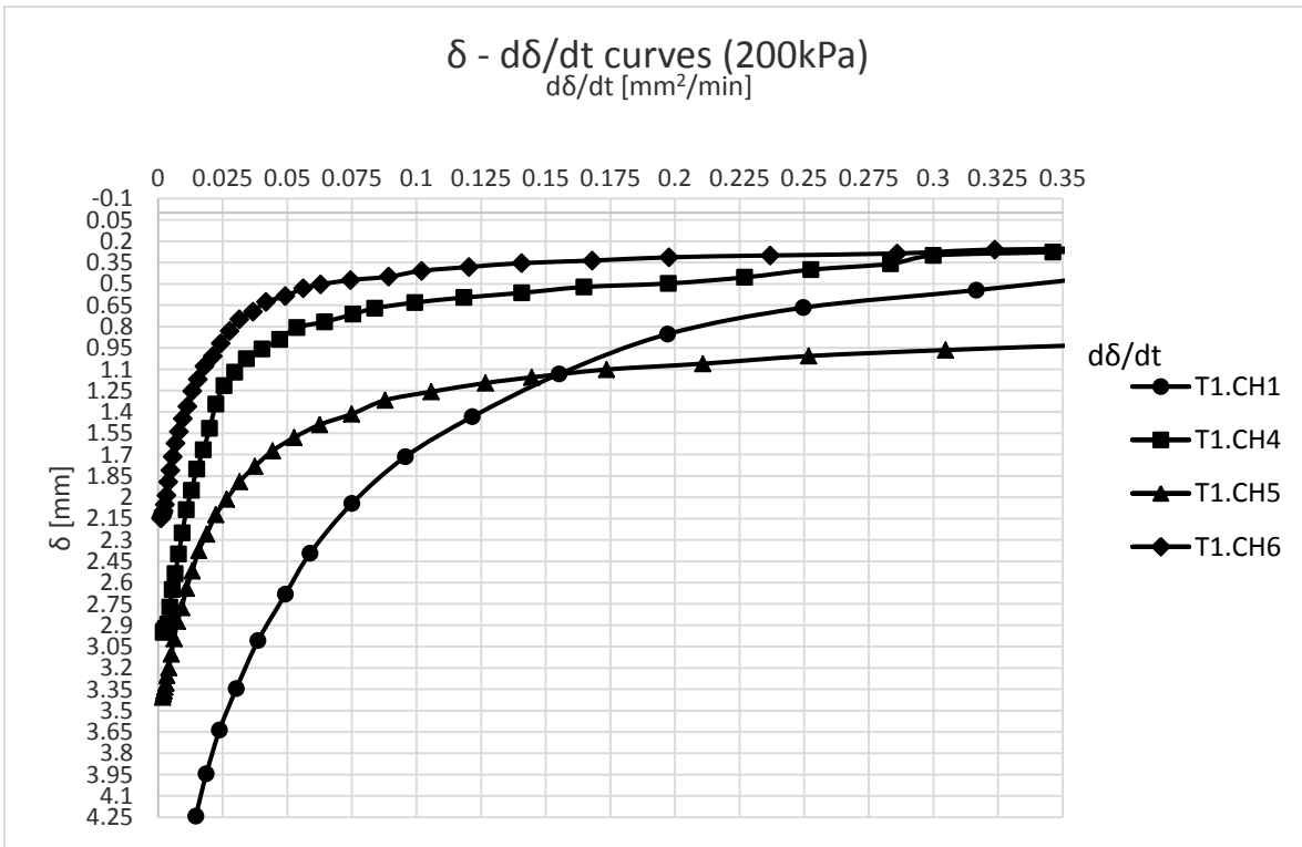
Figure 5: Typical \delta - d\delta/dt curves for reconstituted krakowiec clay.
