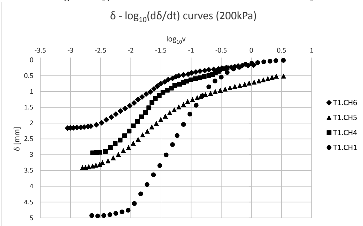
Figure 6: Typical \delta - \log_{10}(d\delta/dt) curves for reconstituted krakowiec clay.
