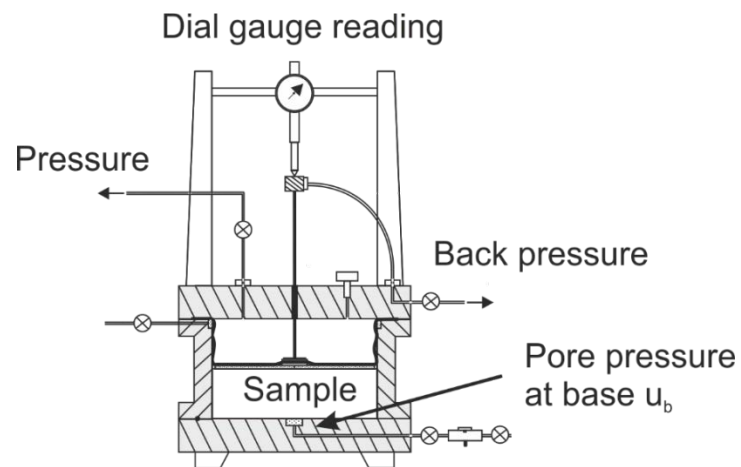
Figure 1: Arrangement of Barden-Rowe cell.
