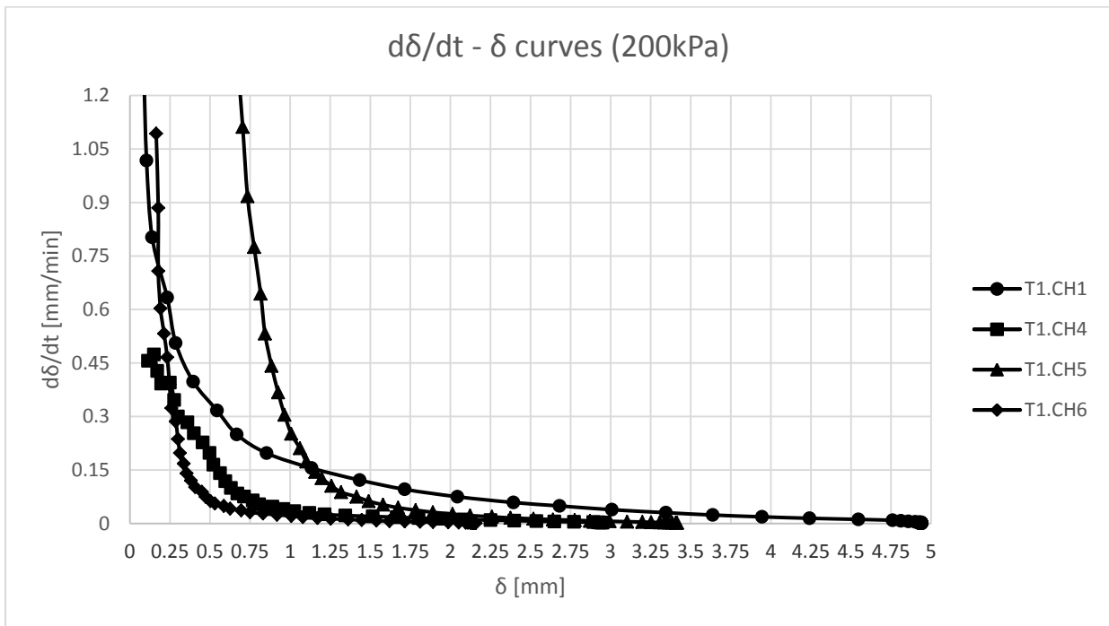
Figure 4: Typical d\delta/dt-\delta curves for reconstituted krakowiec clay.
